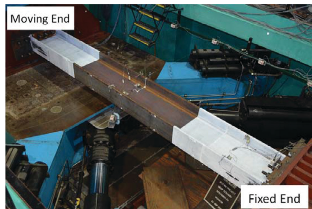
Fig. 2. Test setup.
