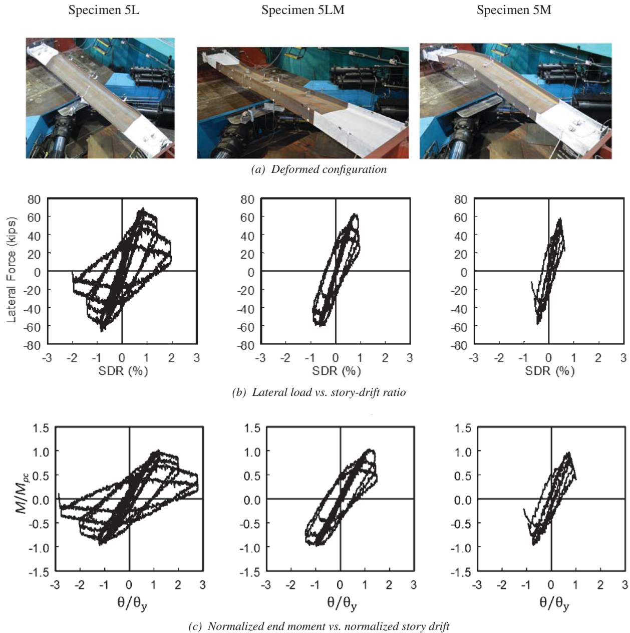
Fig. 9. Group 5 (W24×55 section): Failure mode and hysteresis response.
